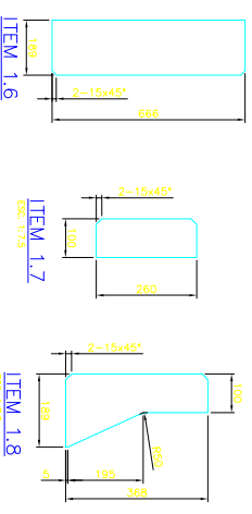
DETAILHE 04
