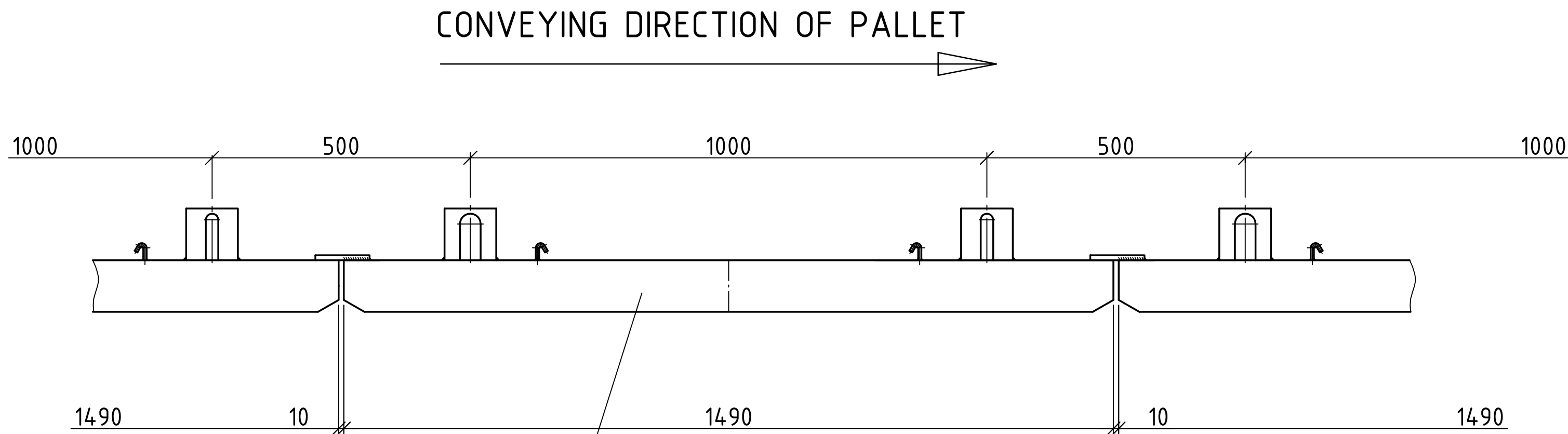
DROP BAR 31,5x1490
