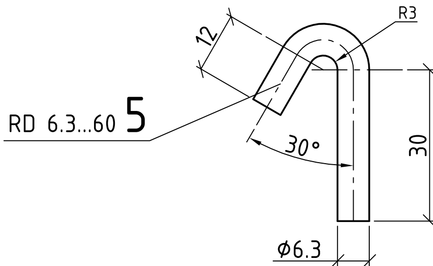
DETAIL X SCALE 1:1
