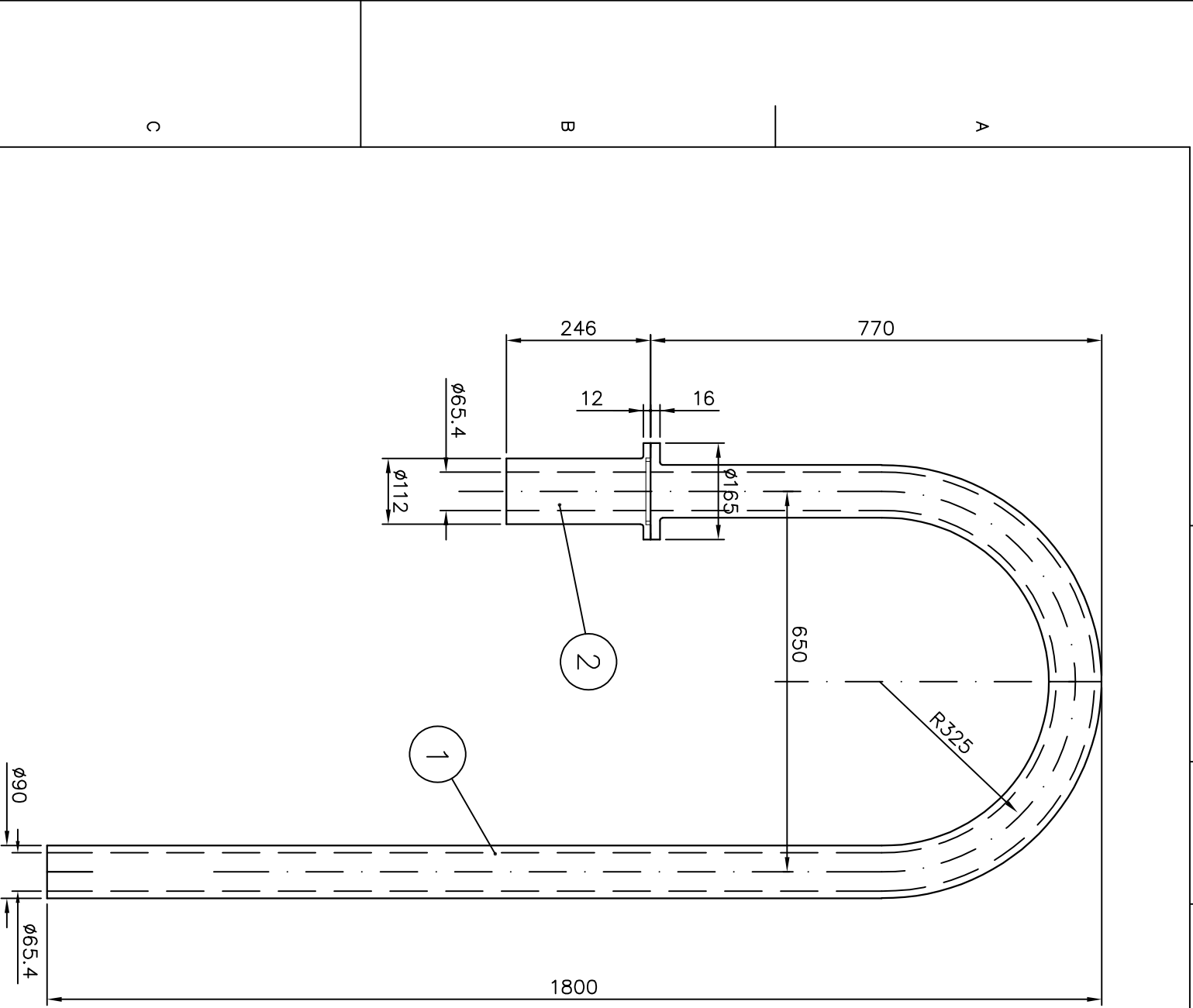
CURVA DE OVER FLOW Ø 3" – PEAD
